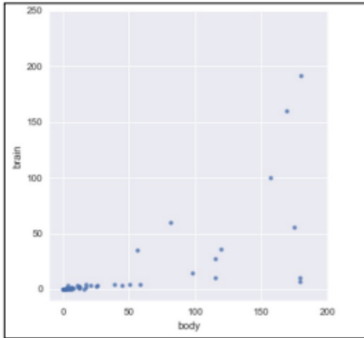
Scatter plot of mammalian brain and body weights
