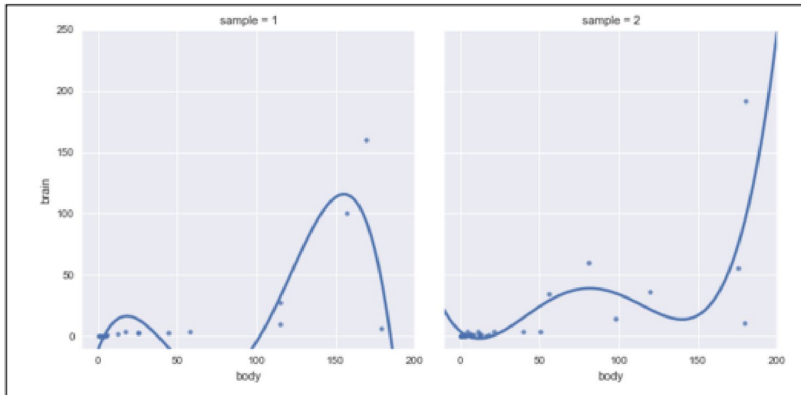
Using a quartic polynomial for regression purposes
